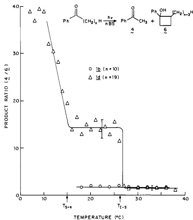
Figure 1. Temperature dependence on the ratio of elimination (4) to cyclization (6) products for photolysis of ketone 1d ( \blacktriangle ) and 1b ( \circ ) in n -butyl stearate. The lines are drawn through points to show the trends in the data only.
