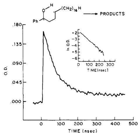
Figure 2. Representative transient absorption decay at 317 nm after laser flash photolysis of 1d at 20 °C in the smectic phase of n -butyl stearate.
